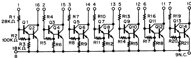
● BA-6250 (7 Transistor Array)
