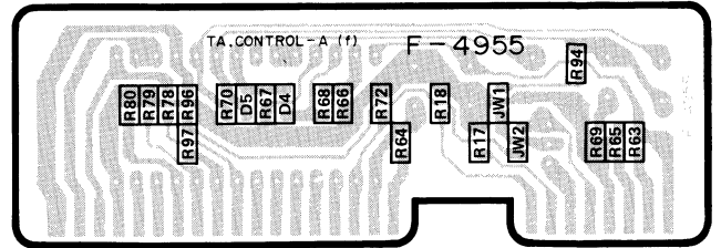
Pattern Side (Chip Parts)
