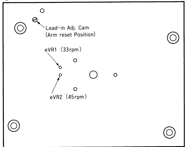
Fig.3-2 Bottom View
