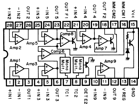
● BA-6150 (Tonearm Servo Control)
