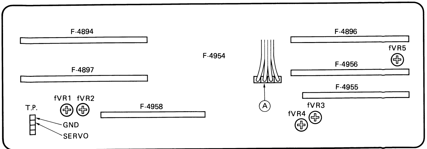
Fig.3-4 F-4954 Test & Adjustment points
