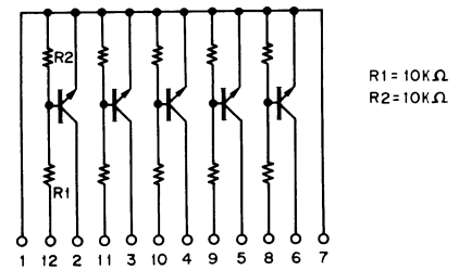
● DT5C114E (5 Transistor Array)
