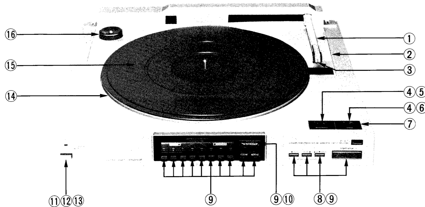
6-2. Front View
